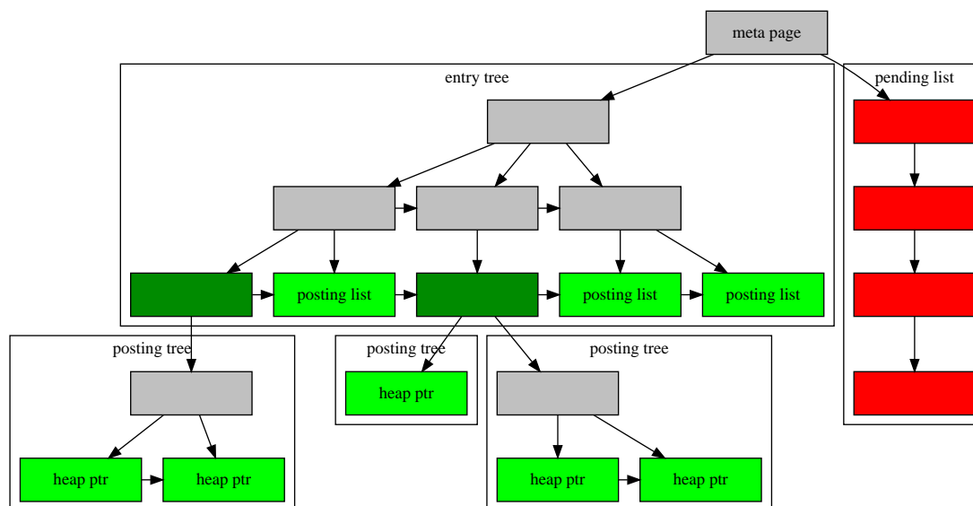
Figure 66.1. GIN Internals
